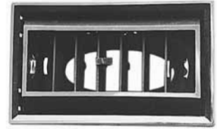
LO-25105 BLACK PLASTIC, PART CHROMED FACE DIMENSIONS: 114mm X 70mm APERTURE: 108mm X 63mm FOUR SNAP-IN CLIPS INCLUDES LS-55130 62mm DUCT ADAPTOR
