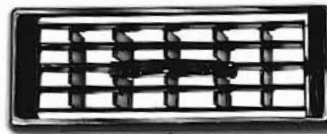
LO-25145 BLACK PLASTIC, PART CHROMED FACE DIMENSIONS: 138mm X 55mm APERTURE: 130mm X 46mm FOUR SNAP-IN CLIPS
