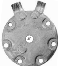
COS-82602 (R134a) VERTICAL O-RING (MIOR) FITS: SD 709, SD7H13/15 SANDEN: 7863-9630
