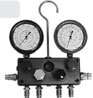
REFCO FRONT WHEEL, 4-WAY, MULTI-REFRIGERANT MANIFOLD. SUPPLIED COMPLETE WITH 1830mm LINES AND R134a COUPLERS.
