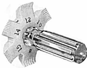
TO-18740 FIN COMB MULTI-HEADED COMB SUITABLE FOR MOST CONDENSER AND EVAPORATOR FINS.
