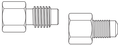
VACUUM PUMP UNIONS 1/4" FEM. FLARE-1/2" MALE ACME TO-77450 1/2" FEM. ACME -1/4" MALE FLARE TO-77475
