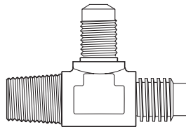
TO-77500 VACUUM PUMP 'T' UNION MALE PIPE - 1/2" MALE ACME - 1/4" MF
